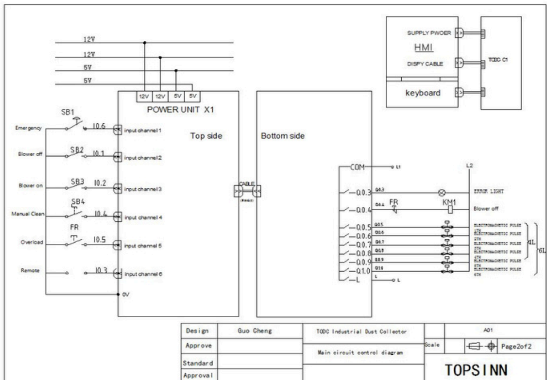
Fig. 28 Control circuit diagram 1 (TODC-4L/6L)
