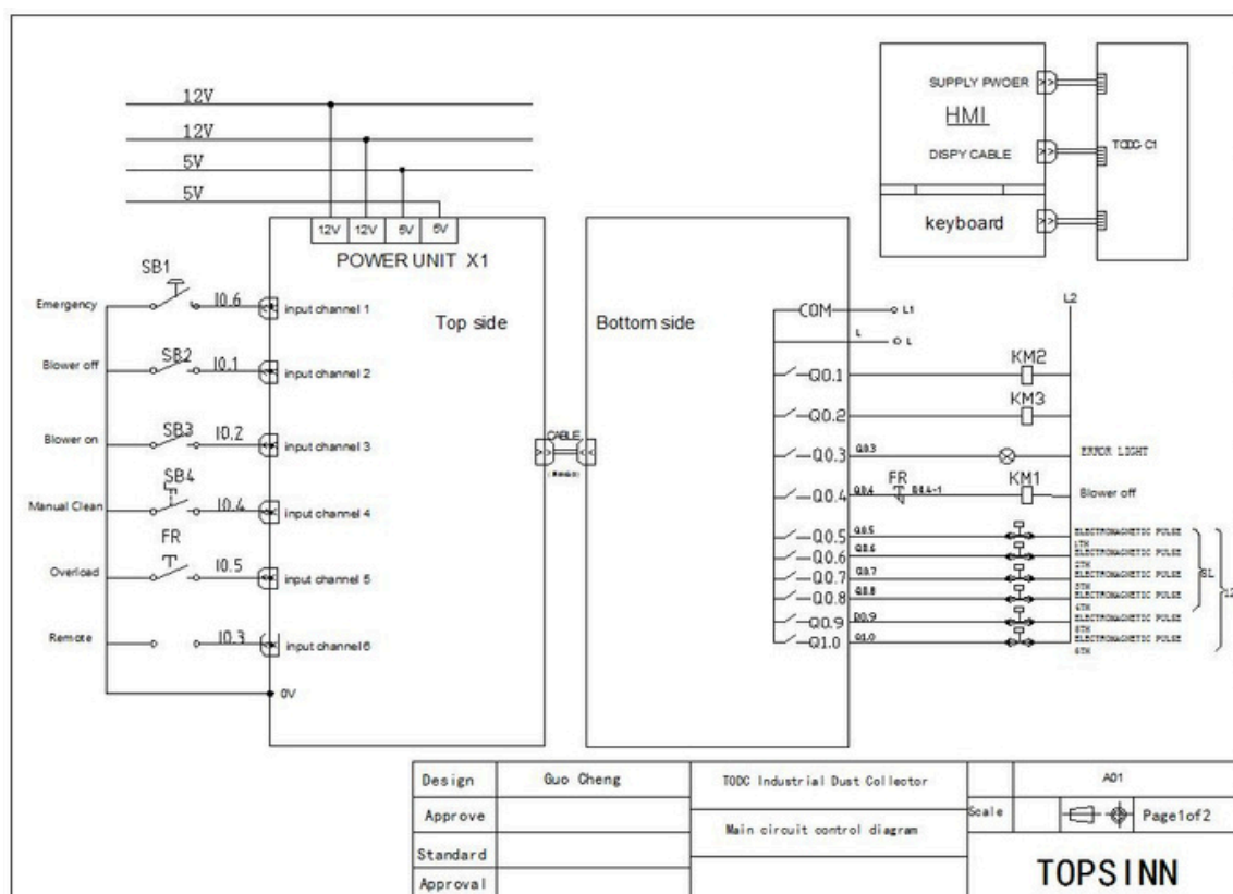
Fig. 29 Control circuit diagram 2 (TODC-8L/12L)
