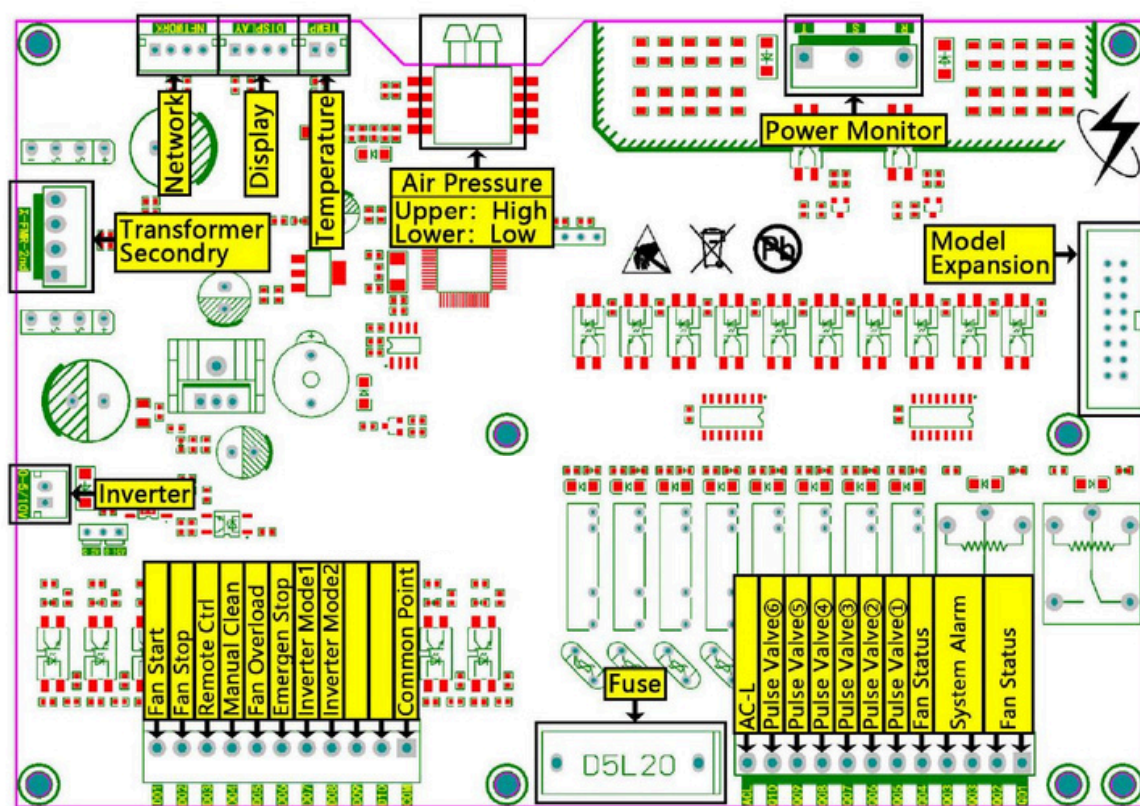
Fig.30 Control panel point bitmap
