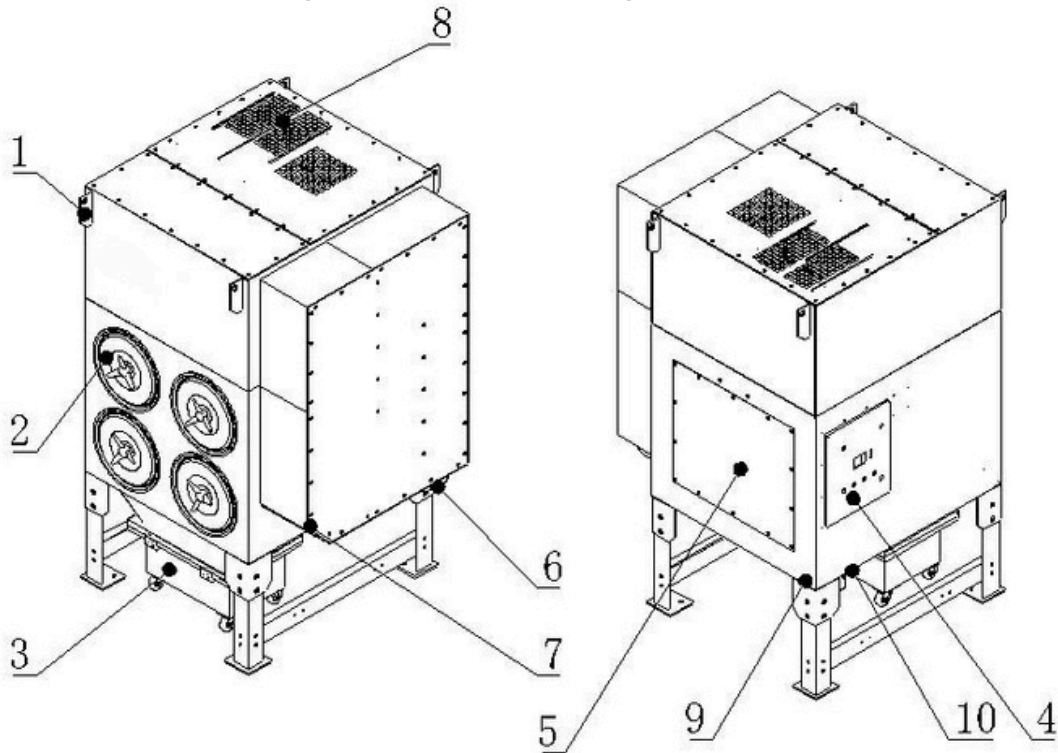
Fig.6 AppearanceDiagram
